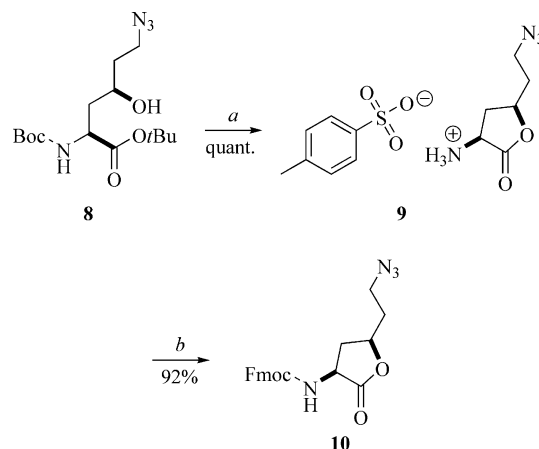
Scheme 3. Reagents and conditions: (a) PTSA, CH 3 CN; (b) FmocOSu, K 2 CO 3 , acetone/H 2 O.
