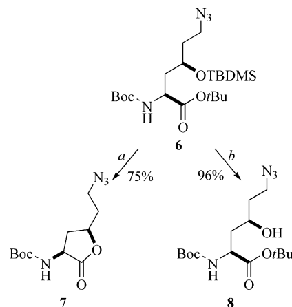
Scheme 2. Reagents and conditions: (a) TBAF, THF; (b) TBAF, AcOH, THF.
